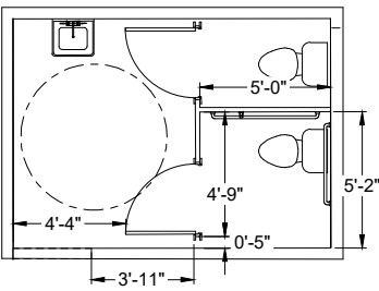
N Family Classroom Toilet Compartment Standards
