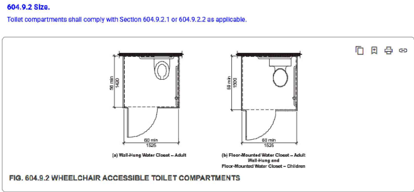
Toilet Compartment size requirements
